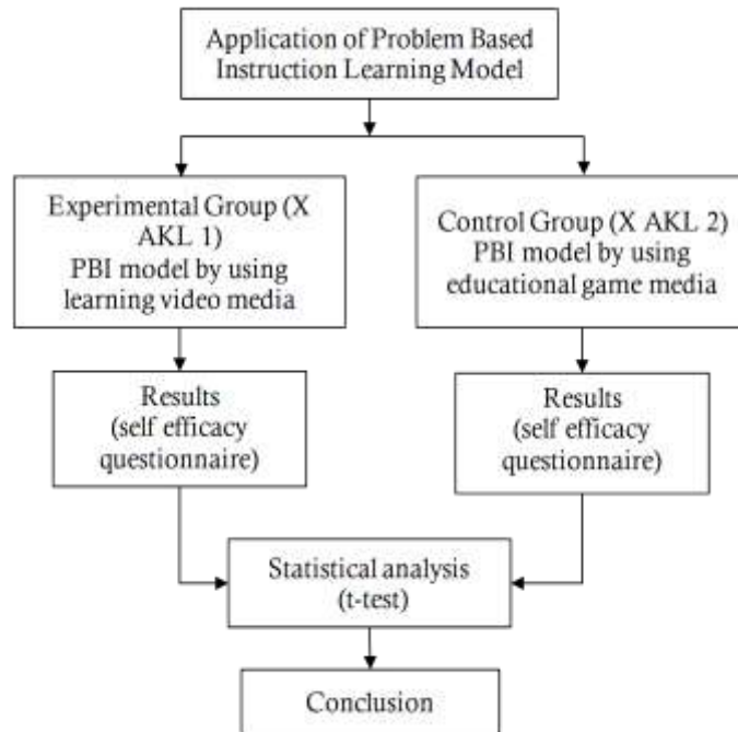
Figure 1. Framework Theory
